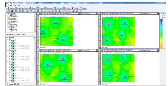
Figure 11: Multi-floor deployments
