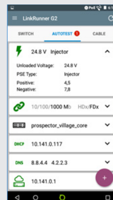
Verify voltage and the cable pairs used by a 24V PoE Injector.
