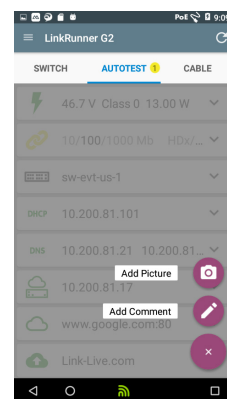
Directly take picture or add comment to the last test result.
