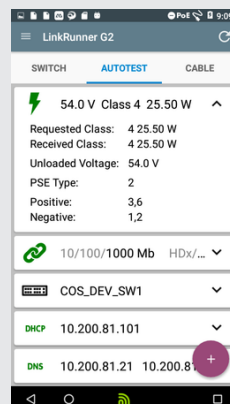
Verify voltage and power from an IEEE 802.3bt Class 8 PSE.
